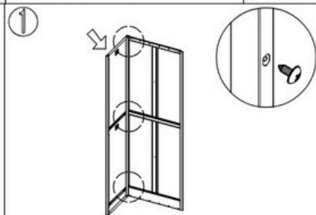
1 Bolt the left side and back plate with self-tapping screws (5x10).
