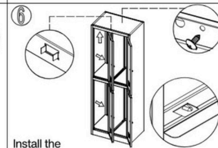
6 Install the top plate, then adjust the upper and lower division plate till fit well.
