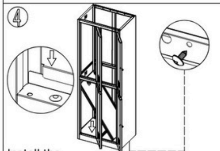
4 Install the bottom plate, then install the lower division plate in the same way.
